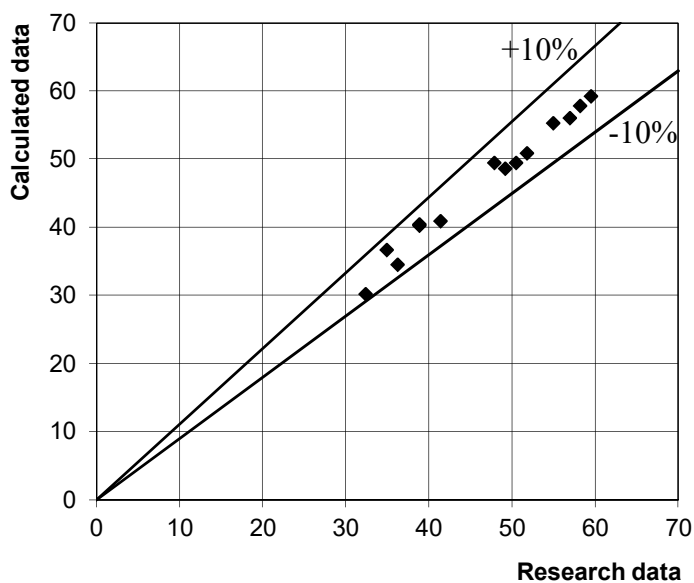
Figure 2. Comparison of calculated and experimental values of h_{cr}^*
