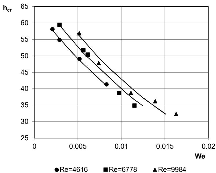
Figure 3. Effect of the We_{01} criterion on the dimensionless height of dispersion onset. Calculated data by formula (6) are shown as lines, and experimental data are shown as points for corresponding Re values.
