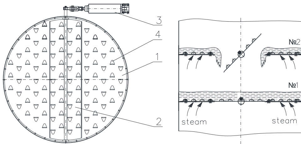
Figure 2. Cyclic mass-exchange plate with a variable free cross-section 1 – plate web; 2 – movable segment; 3 – drive mechanism; 4 – scales
