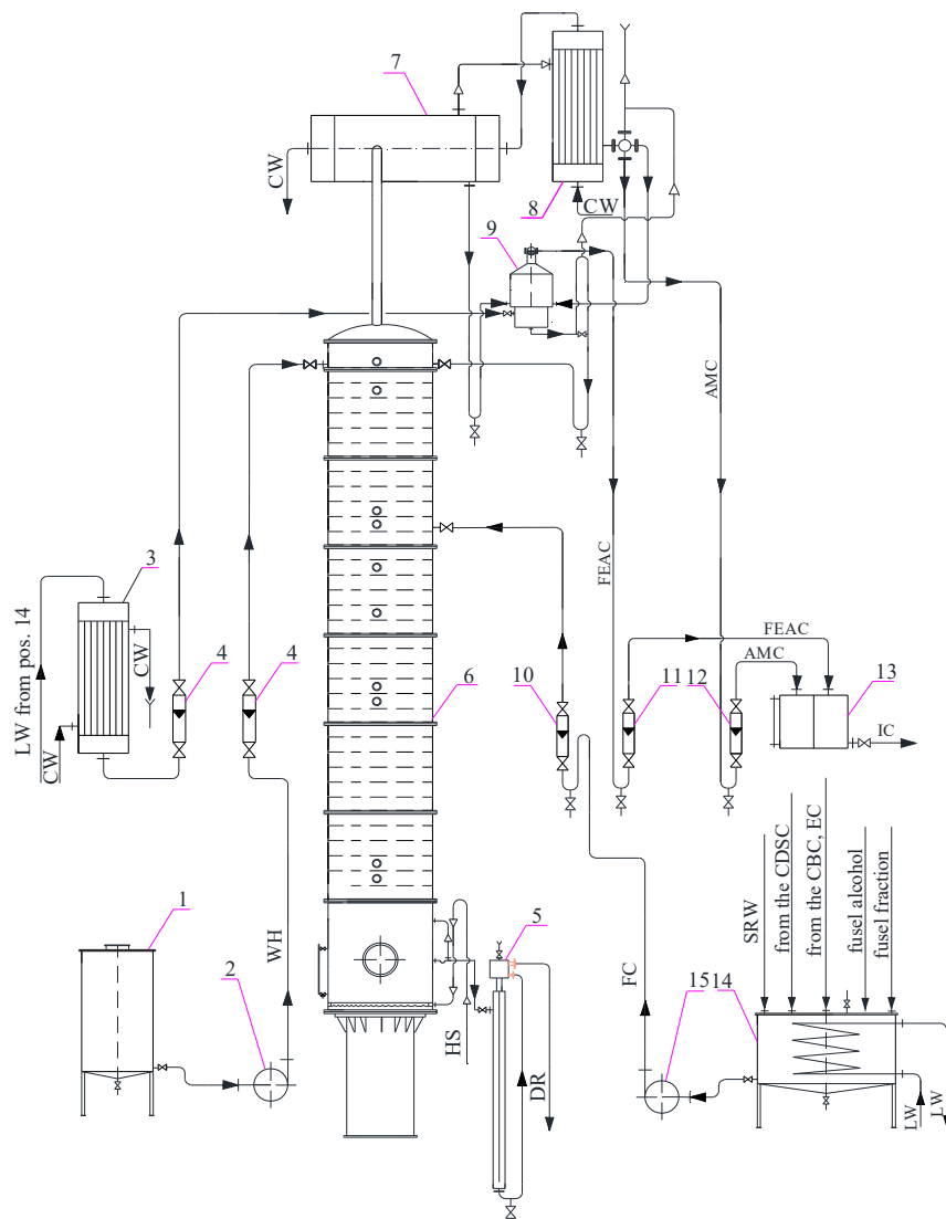
Figure 5. Unit for joint processing of head and fusel fractions by method III 1 – water container; 2,15 – centrifugal pumps; 3 – cooler; 4,10,11,12 – flowmeters; 5 – hydraulic shutter; 6 – impurity concentration column; 7 – dephlegmator; 8 – condenser; 9 – decanter; 13 – impurity concentrate container; 14 – alcohol-containing fraction container.
