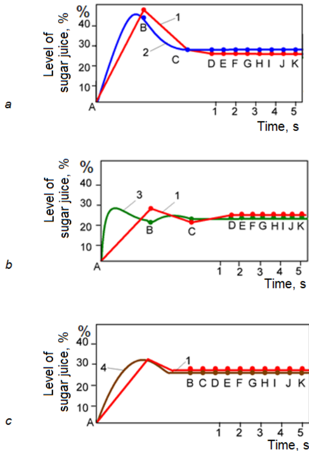
Figure 4. Comparison of transients of forecasted and actual levels of sugar juice in the first body of the evaporating station using:
